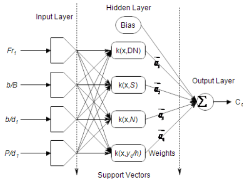
Figure 5. The network architecture of SVM
