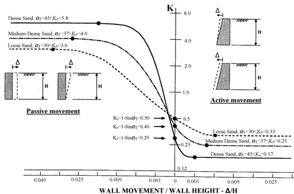
Figure 2. Earth pressure coefficient versus relative wall displacement (NCHRP 1991) [25]
