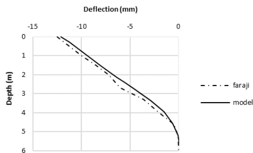
Figure 3. Abutment deflection in the models of Ting & Faraji and also the present study
