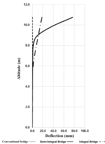
Figure 4. Abutment's deflection with passive soil
