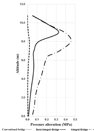
Figure 7. Soil pressure-drop pattern in abutments with active soil
