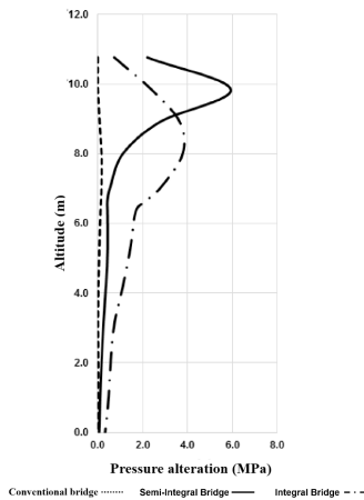
Figure 6. Soil pressure-rise pattern in abutments with passive soil
