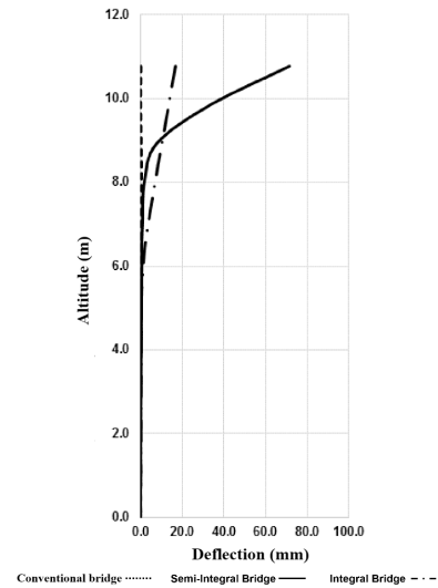
Figure 5. Abutment's deflection with active soil
