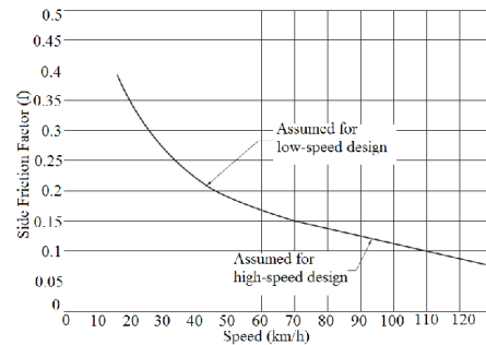
Figure 2. Side friction Demand factor assumed for design [4]
