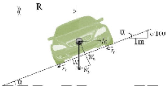
Figure 1. Cornering vehicle forces in PM model
