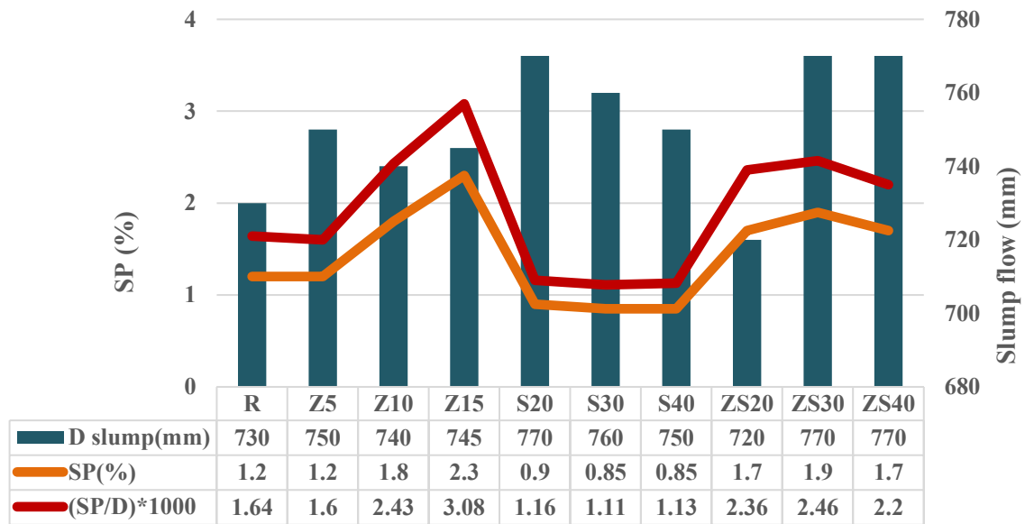
Fig. 3. Slump flow diameter and HRWR demand rate.
