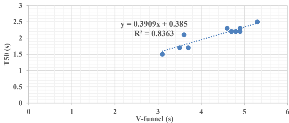
Fig. 5. Relationship between T50 and V-funnel flow times.
