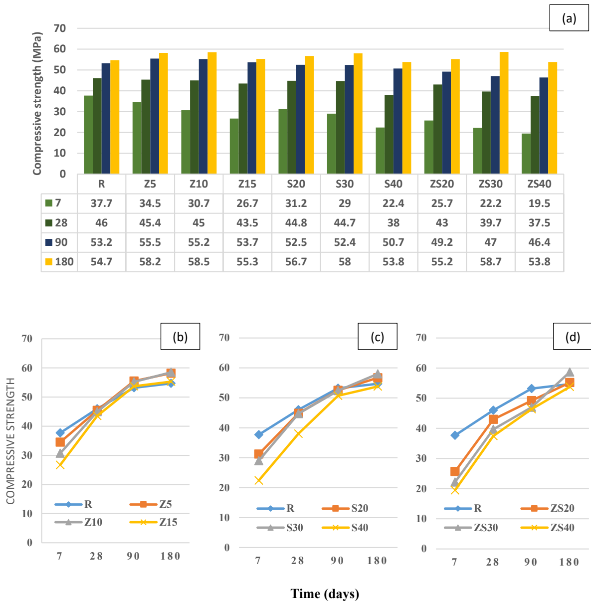
Fig. 6. Compressive strength of SCC mixtures made with various SCMs (MPa).
