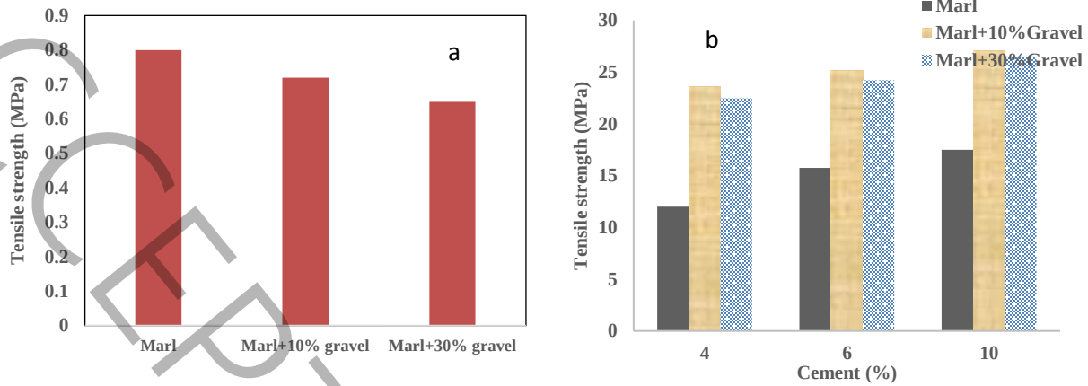
Fig. 9. Variations in Indirect Tensile Strength of Studied Samples: (A) Effect of Gravel on Marl Indirect Tensile Strength, (B) Effect of Cement on Indirect Tensile Strength of Marl and Gravel Mixture after 28 Days of Curing.
