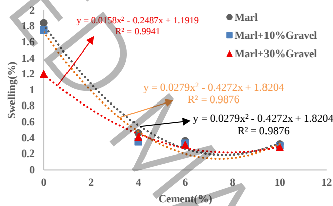
Fig. 7. The influence of cement on the swelling rate of the Marl and Gravel mixture after 28 days of curing.
