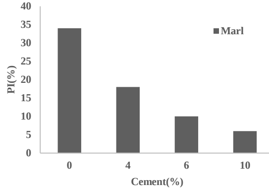
Fig. 4. Effect of Cement on the Plasticity Index of the argillaceous Marl.
