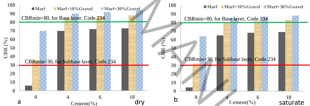
Fig. 6. Influence of cement stabilization on the California Bearing Ratio (CBR) performance of Marl–Gravel mixtures after 28 days of curing under: (a) dry loading conditions, and (b) saturated loading conditions.
