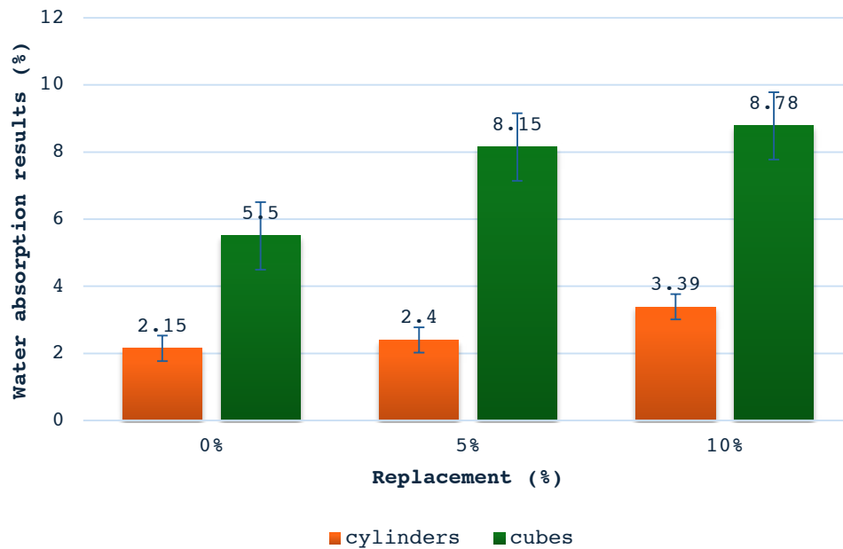
Fig. 4. Water absorption results.
