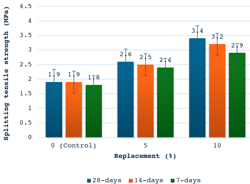
Fig. 3. Splitting tensile strength results.
