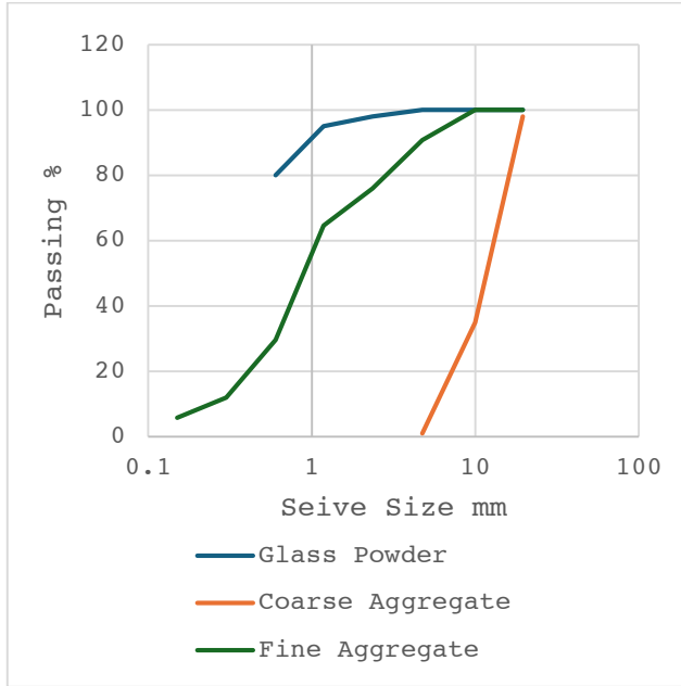
Fig. 1. Particle size distribution curves of the constituent materials.
