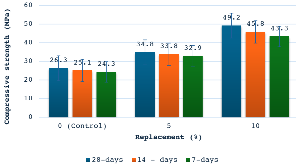
Fig. 2. Compressive strength results.
